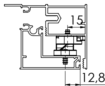
SAPA - ECO FACADE
