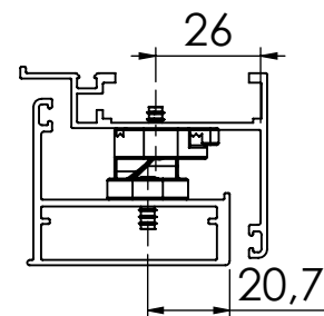
SAPA - ECO FACADE
