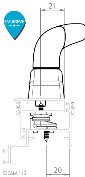
FACHADA GRID (HYDRO)
