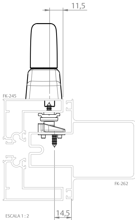
FACHADA STICK (OLGA COLOR)
