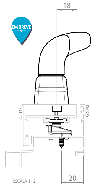
FACHADA GRID (HYDRO)
