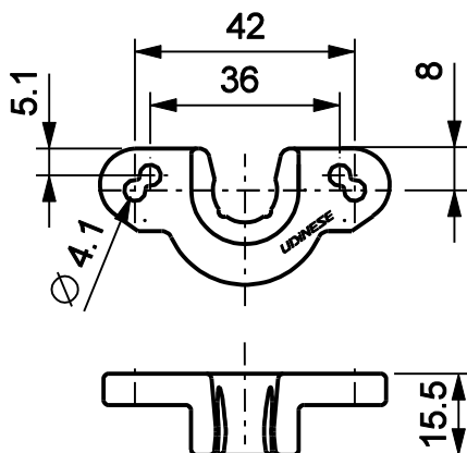
Mancal
