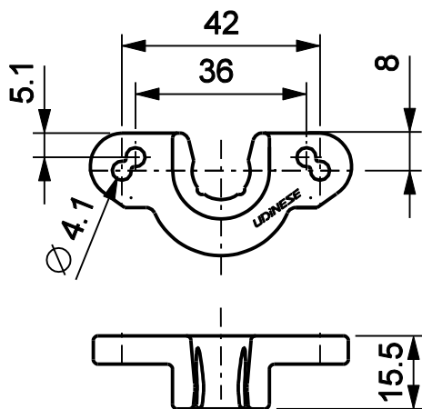
Mancal
